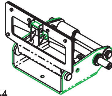
ITEM 44 FM-26-XXX-EZ ROCKER BLADE W/TAB CUTTER SUB-ASSY
